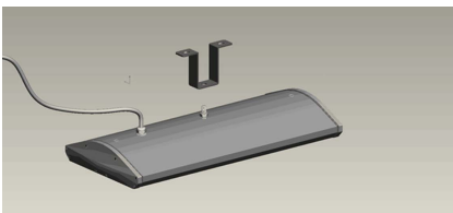
Surface mount with bracket and dimming wire
