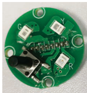
Image: Indicator light LED and Tact Switch
