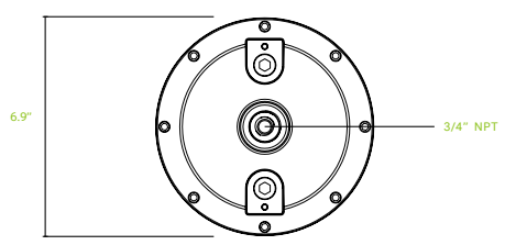
Ceiling Mounting Plate
