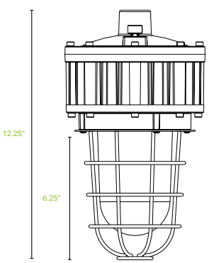
Drop Lens with Wire Guard w/ Pendant Mount
