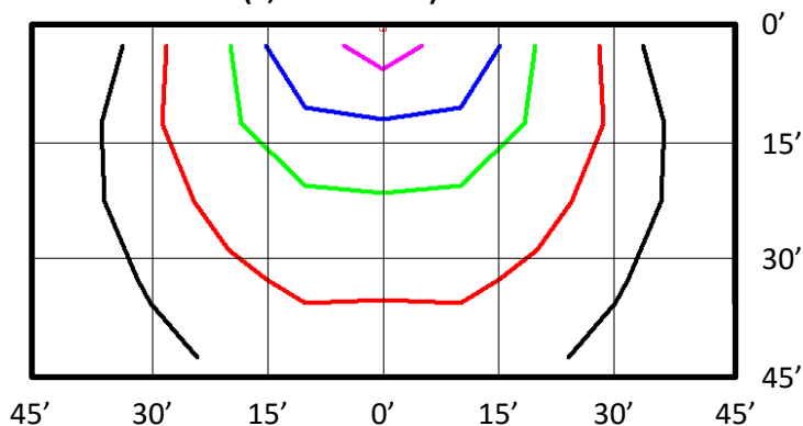
FLEDWP30W-4K (2,747 Lumens)
