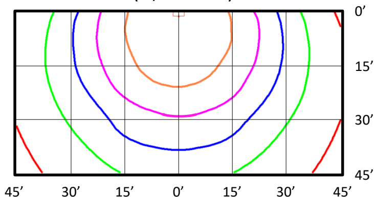
FWP120SN-5K-PRM (15,787 Lumens)
