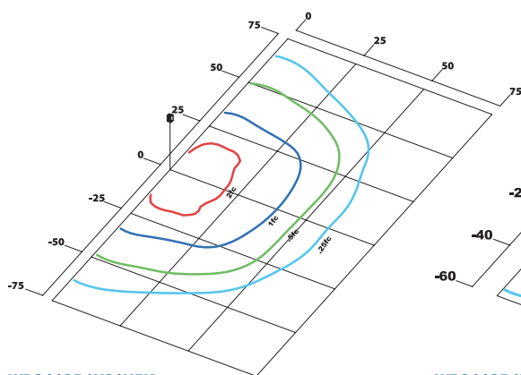
WPC44QD1X81U5K Type IV Grid in MH MH=25 Feet
