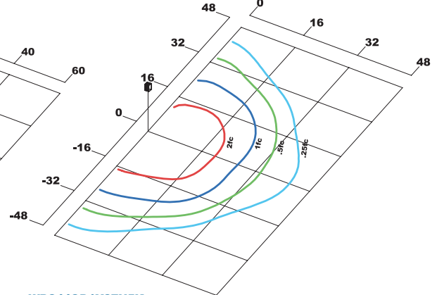
WPC44QD1X37U5K Type IV Grid in MH MH=16 Feet
