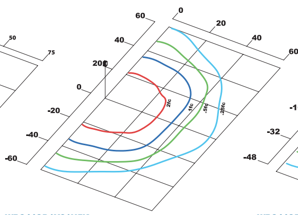
WPC44QD1X81U5K Type IV Grid in MH MH=20 Feet
