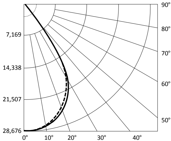
JGMPALPRO240-4K-MW (30,937 Lumens, Medium Wide)
