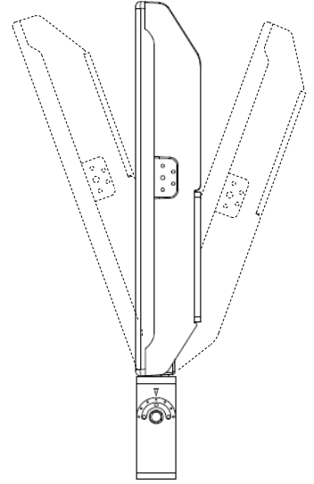
Trunnion Mount JGMPALPRO -TR-80/280
