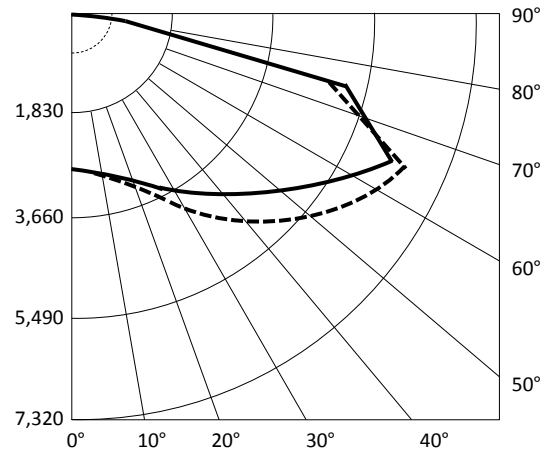
JGMPALPRO240-4K-VW (27,944 Lumens, Very Wide)
