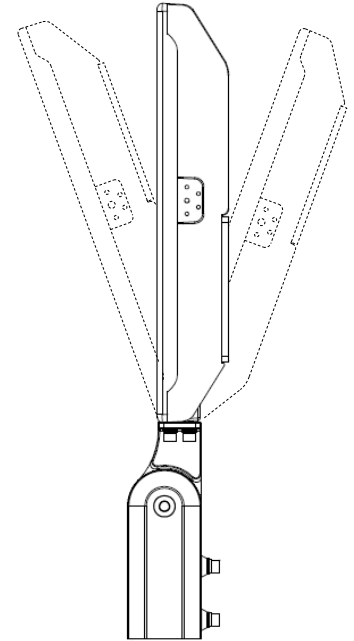
Slip-Fitter Mount JGMPALPRO -SF-80/280
