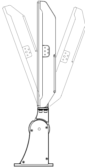
Adjustable Arm Mount JGMPALPRO -ARM-80/280
