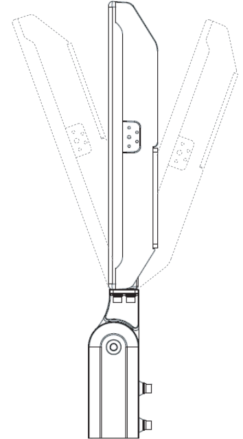
Slip-Fitter Mount JGMPPAL-SF-80/280
