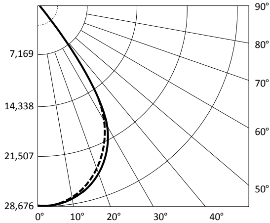
JGMPPAL240-4K-MW (30,937 Lumens, Medium Wide)
