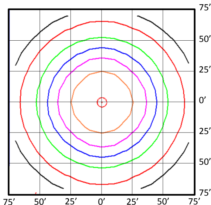
VICOHBR32-4K-B-UNV (32,727 Lumens)
