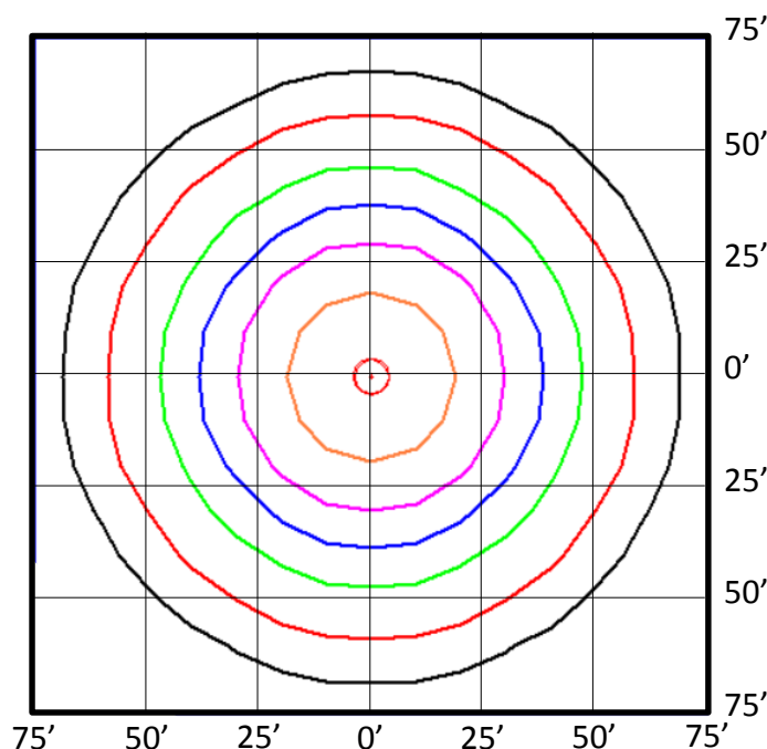
VICOHBR21-4K-B-UNV (20,799 Lumens)
