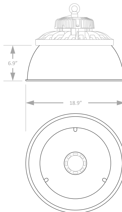
VICOHBRN-ACLREFL90-PRM Acrylic Reflector, 90° Beam Spread
