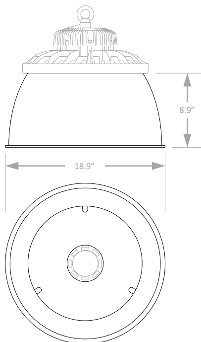
VICOHBRN-ACLREFL60-PRM Acrylic Reflector, 60° Beam Spread
