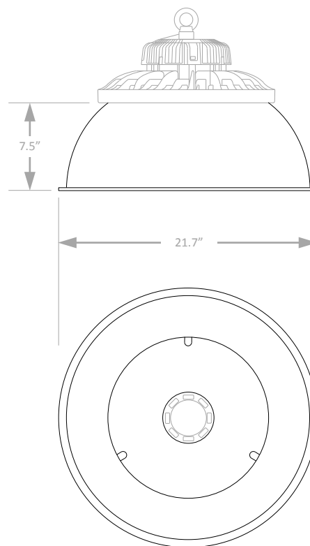
VICOHBRN-ALMREFL90WIDE-PRM Aluminum Reflector, 90° Beam Spread
