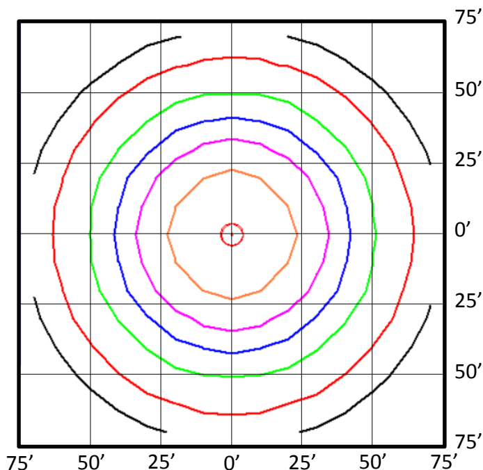
VICOHBR27-4K-B-UNV (27,415 Lumens)
