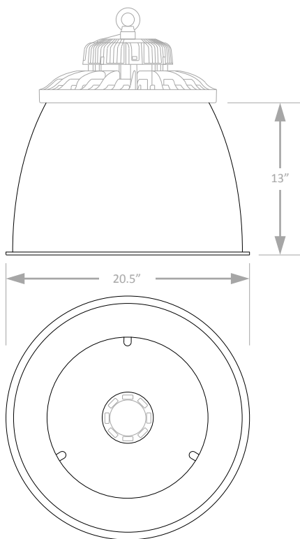
VICOHBRN-ALMREFL60-PRM Aluminum Reflector, 60° Beam Spread
